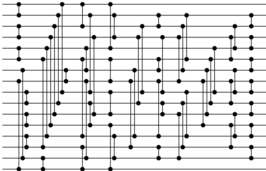
Figure 1: Sorting network with 63 comparators in 10 stages.
